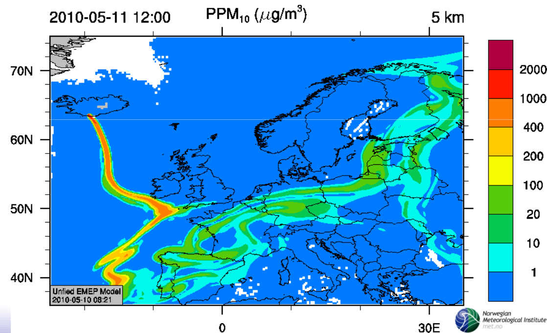
Modelling eruption of the Eyjafjallajökull volcano (2010)
