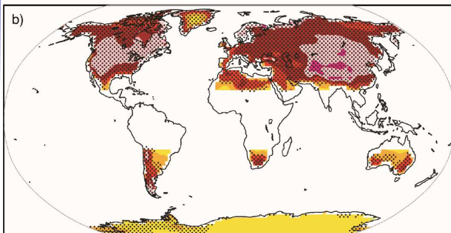
Days with frost
