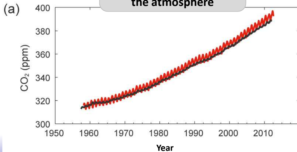
Changes in carbon dioxide concentration in the atmosphere
