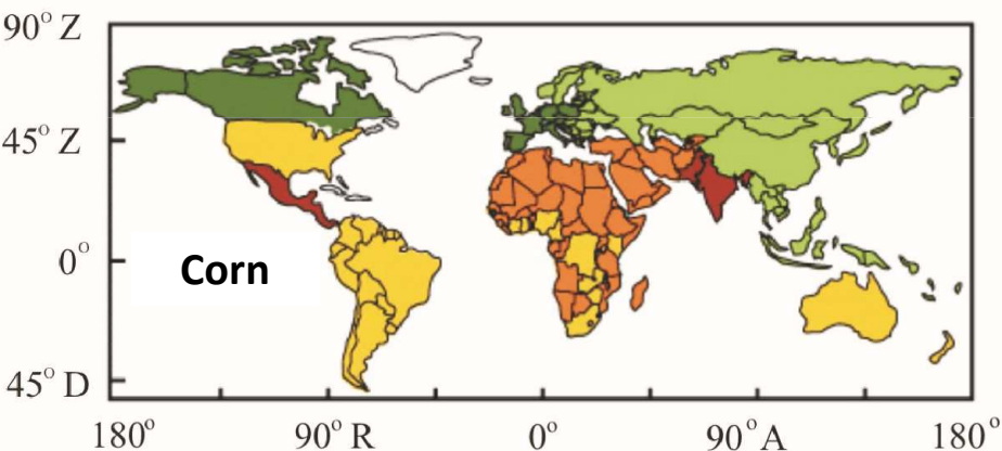
Changes in crop yields in 2050 (%)
