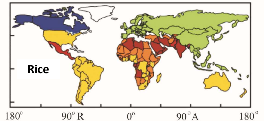
Changes in crop yields in 2050 (%)
